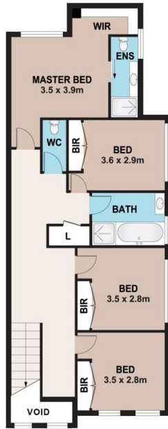
FIRST FLOOR
